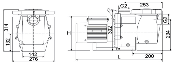
Self-Priming Pump
