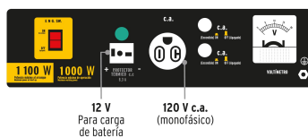
Panel de control GEN-10P
