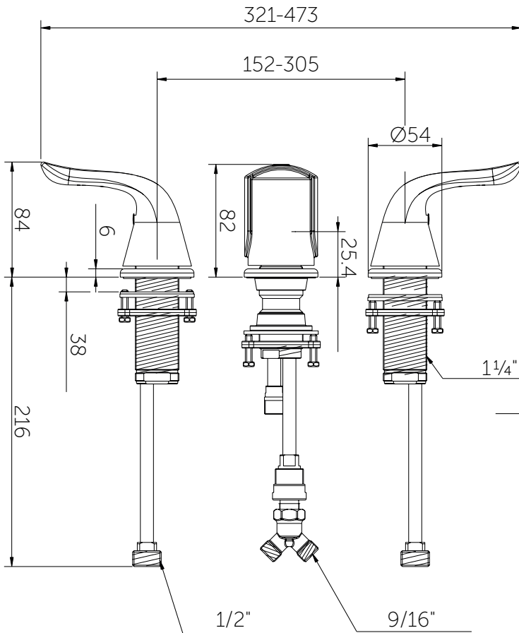
VISTA FRONTAL / FRONT VIEW
